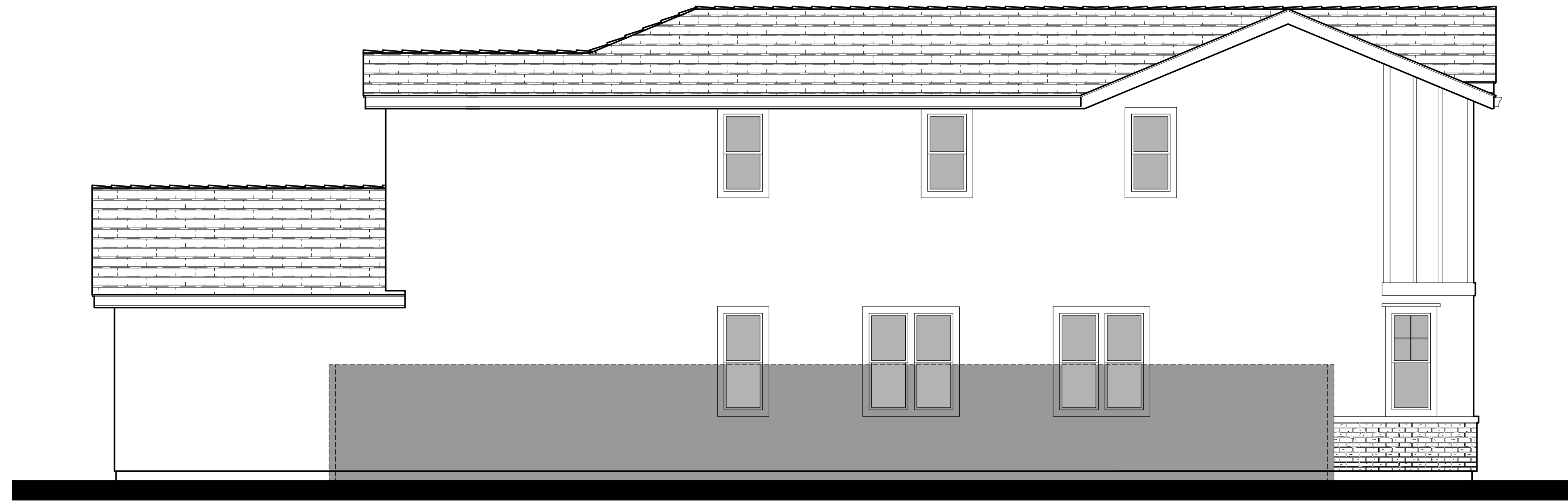
Left Elevation
