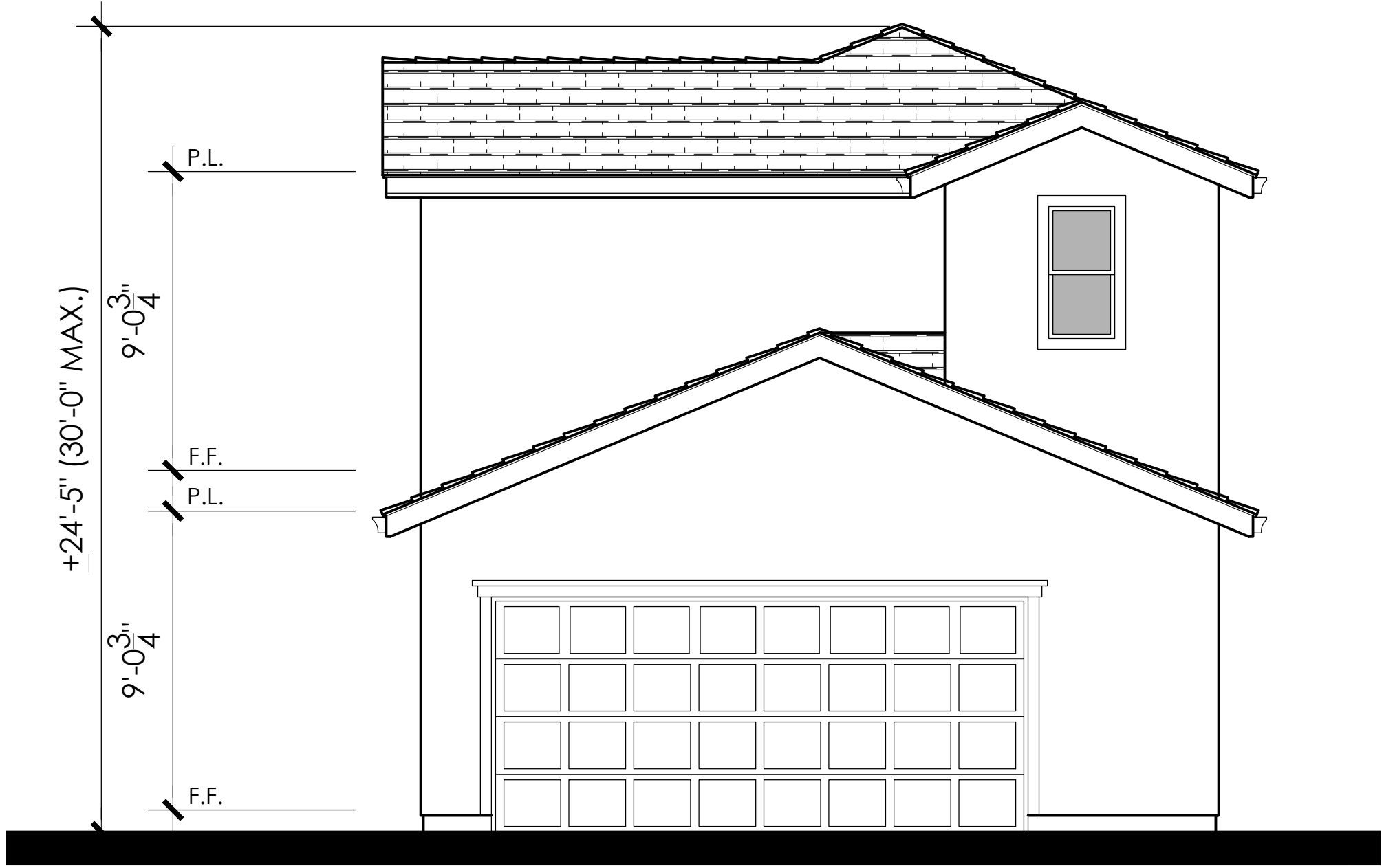
Rear Elevation
