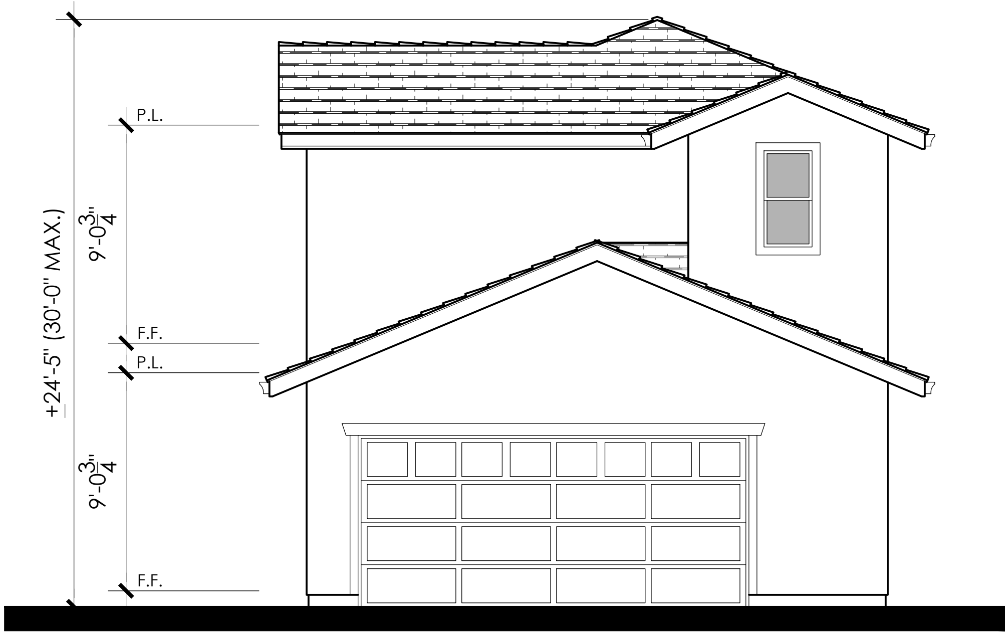
Rear Elevation
