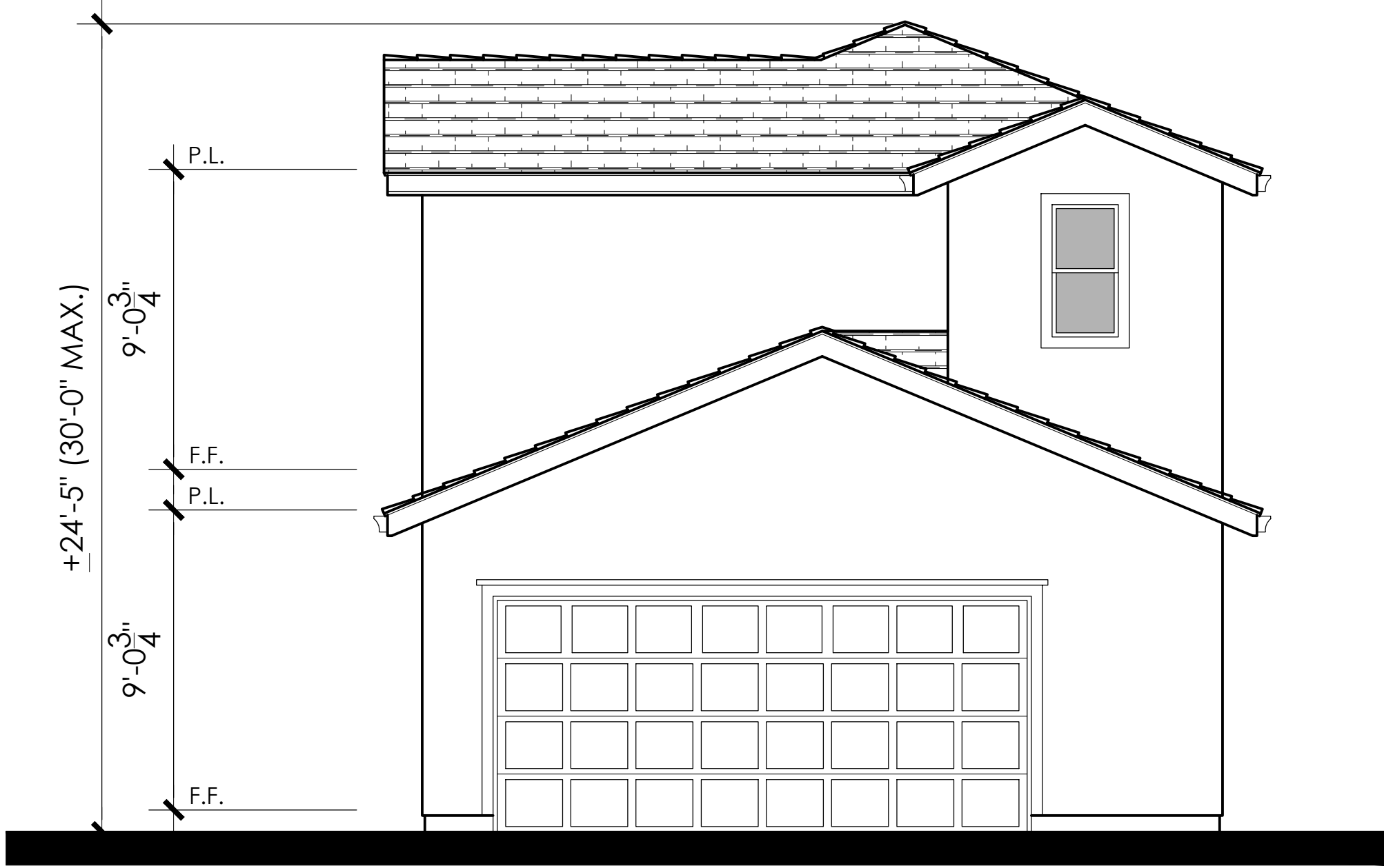
Rear Elevation
